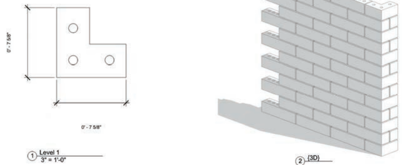
Figure 3: Occhiato University Center shop drawing of special shape return brick generated by Revit model
