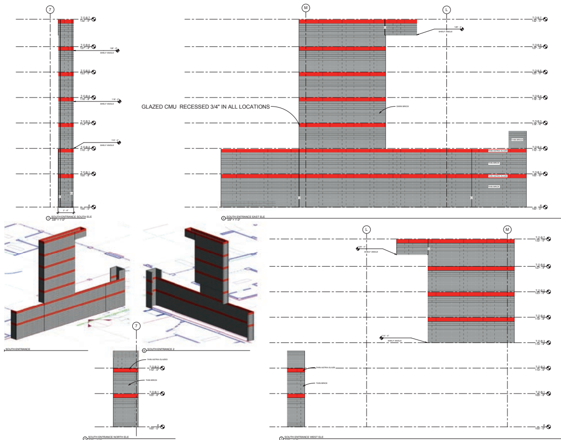
Figure 2: Occhiato University Center 2D and 3D drawings generated from the Revit Model showing brick and Astra Glaze CMU locations and layout
