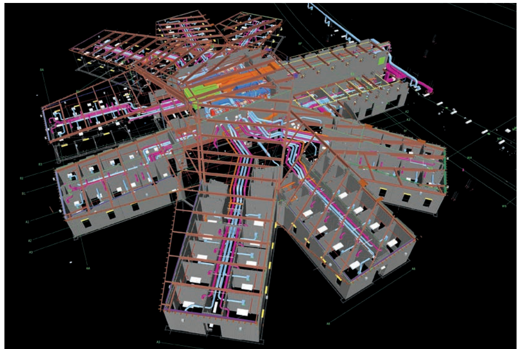
Figure 15: Fulton Mental Health Clash Detection all wings by Navisworks
