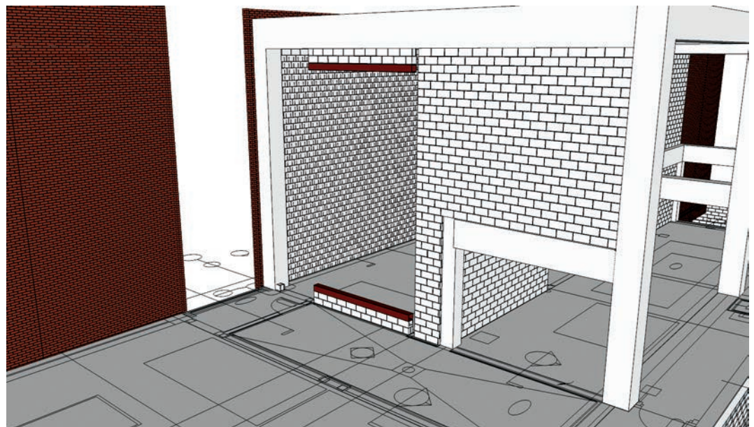
Figure 8: WMH 3D model showing Acoustic CMU and regular CMU interface with concrete structure showing bond and layout
