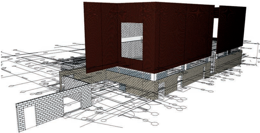
Figure 7: WMH 3D SketchUp model showing Burnished CMU, Brick and CMU back up shows layout and bond
