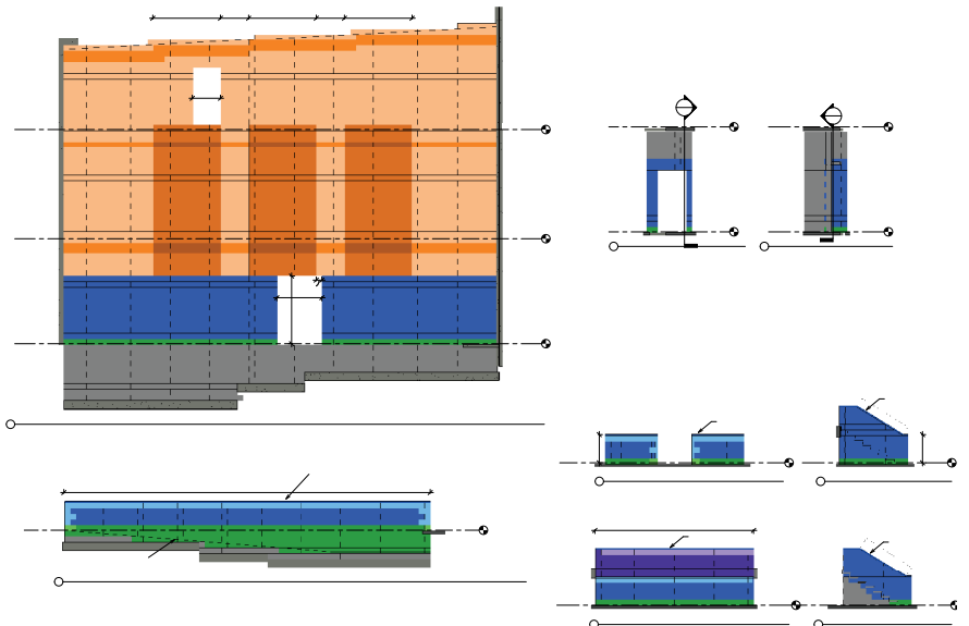
Figure 5: Washington High School 2D lift drawing showing CMU types and layout generated from Revit model
