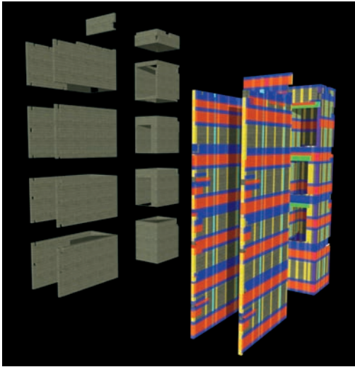
Figure 12: St. Camillus 3D model showing grout, rebar and bond beams generated by Revit model
