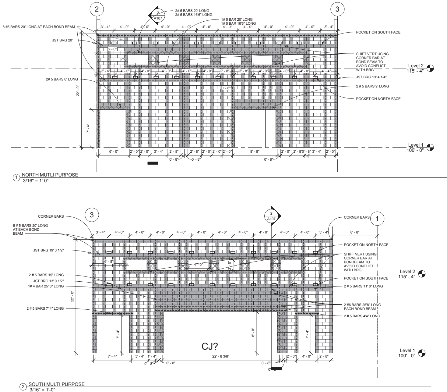
Figure 1: S.E. Health Group Building Expansion 2D lift drawings generated by Revit model showing grout, rebar, bond beam and joist pocket locations
