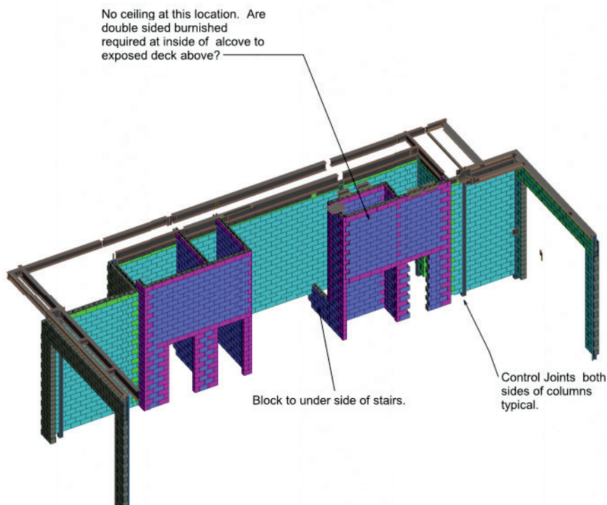
Figure 6: Washington High School 3D model showing different CMU types and locations generated by Revit model
