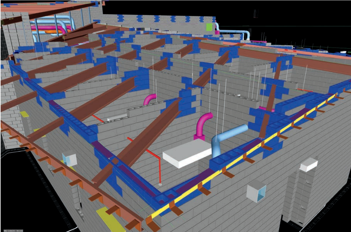
Figure 14: Fulton Mental Health 3D Model showing CMU and Steel interaction generated by CAD BLOX
