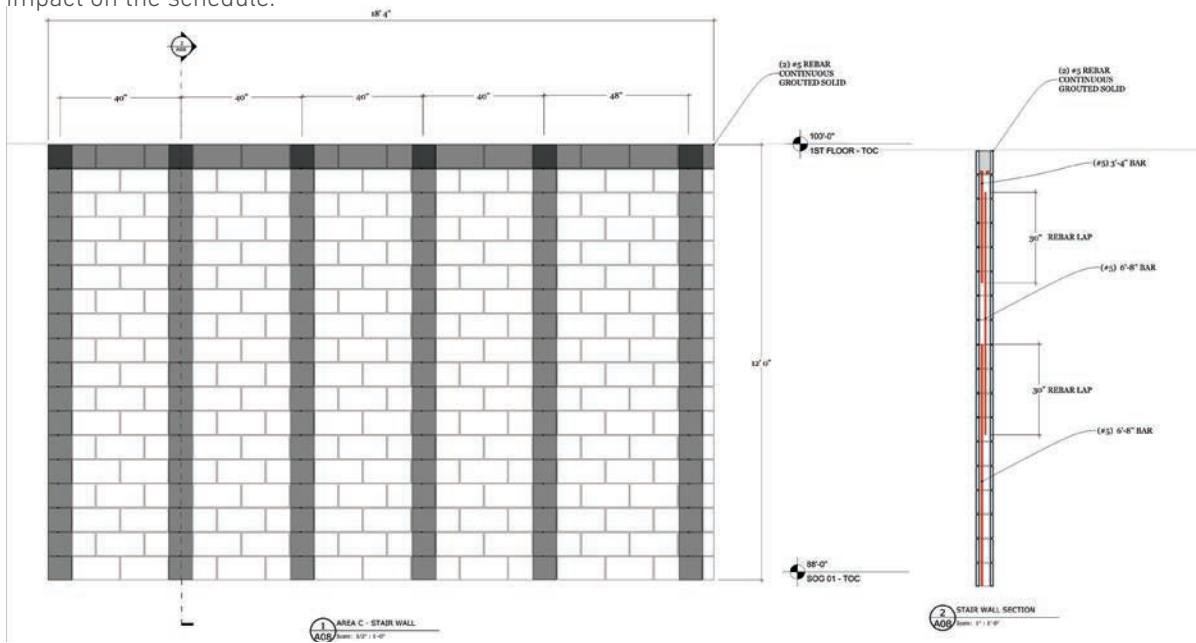
Figure 9: St. Augustine 2D lift drawing showing grout, rebar and bond beam locations generated from 3D SketchUp model
