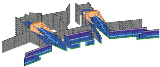
Figure 4: Washington High School 3D model showing different CMU types and locations generated by Revit model
