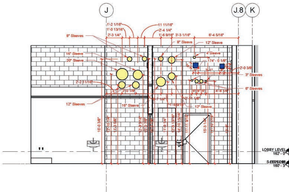
4 H-1225 Corridor-West Elevation 1/4" = 1'-0"
